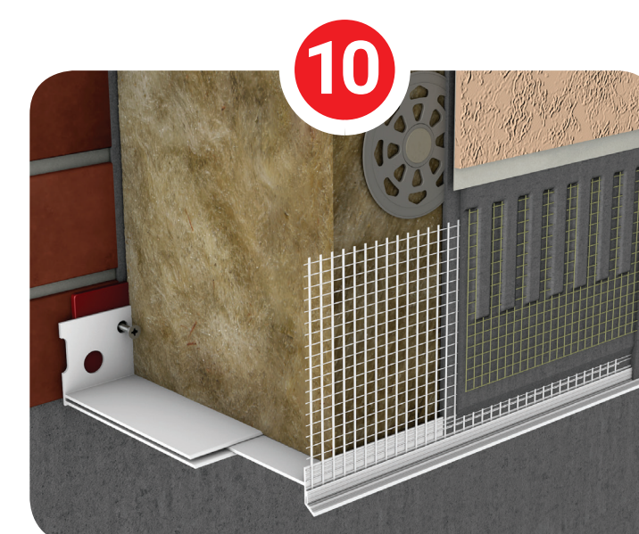
EB PVC VARIO PVC cokola profila komplekts, 2.0 m
