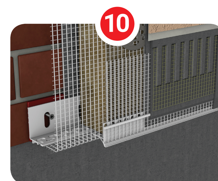
EB PVC PVC cokola profils, 2.0 m
